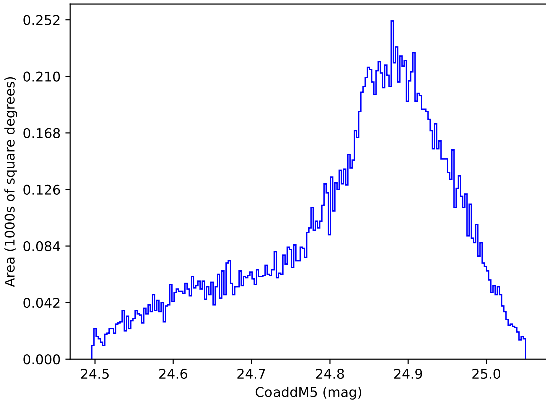
roll_pause_mjdp0_v3.4_10yrs WFD y band: CoaddM5
