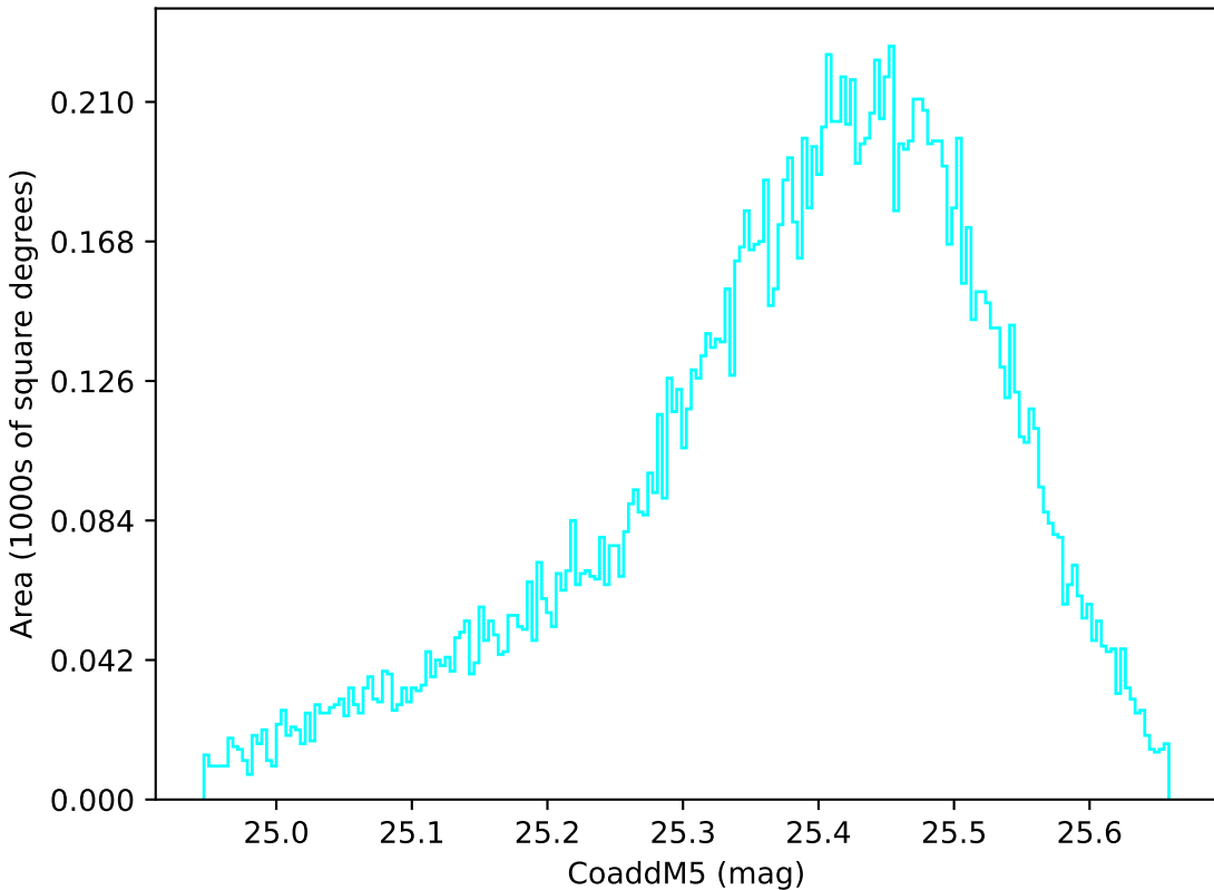
roll_pause_mjdp0_v3.4_10yrs WFD u band: CoaddM5
