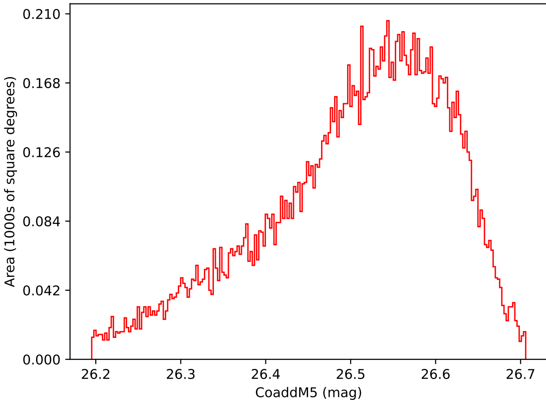
roll_pause_mjdp0_v3.4_10yrs WFD i band: CoaddM5
