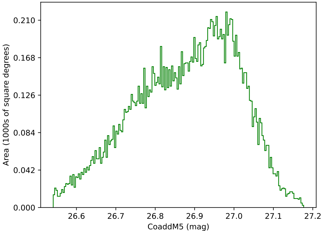
roll_pause_mjdp0_v3.4_10yrs WFD g band: CoaddM5
