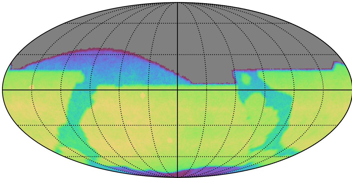
roll_pause_mjdp0_v3.4_10yrs All sky z band: CoaddM5
