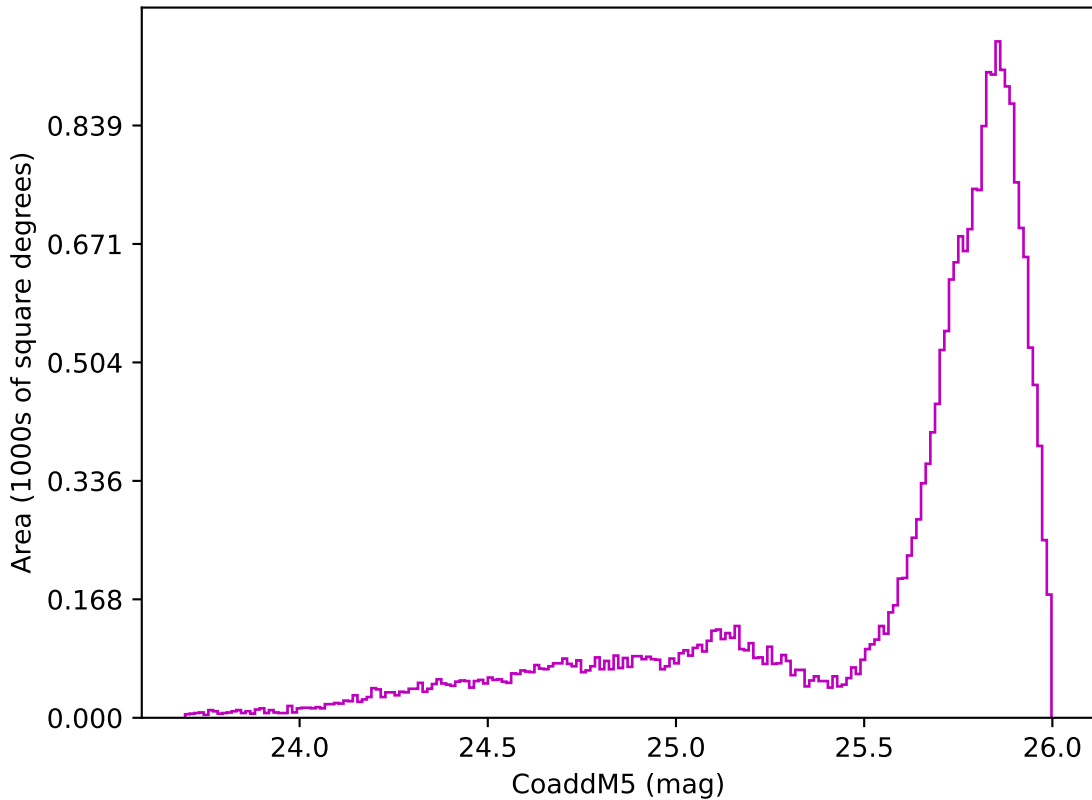
roll_pause_mjdp0_v3.4_10yrs All sky z band: CoaddM5
