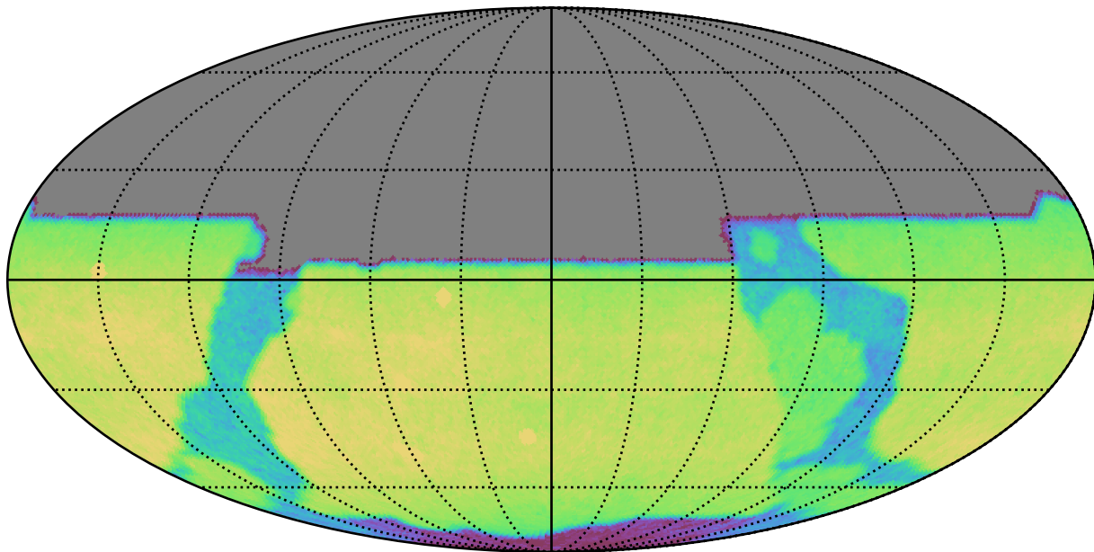
roll_pause_mjdp0_v3.4_10yrs All sky y band: CoaddM5
