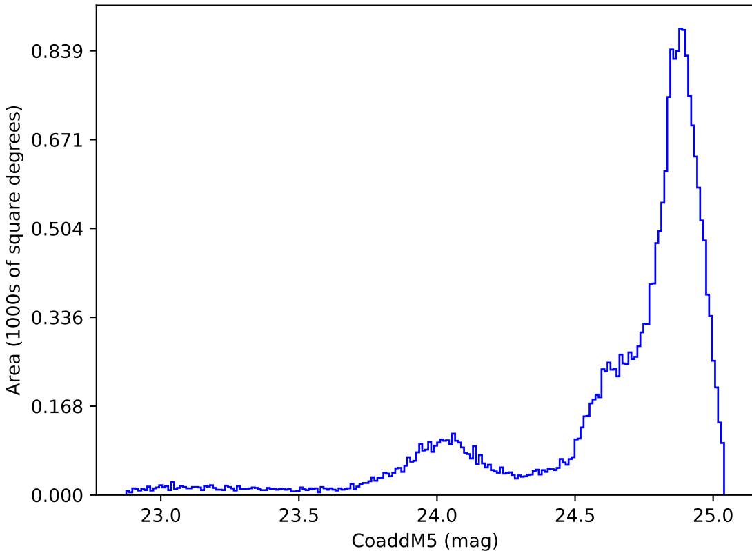
roll_pause_mjdp0_v3.4_10yrs All sky y band: CoaddM5
