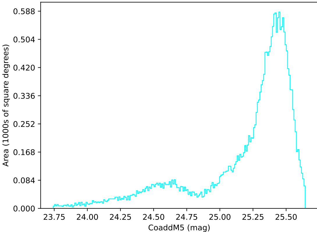
roll_pause_mjdp0_v3.4_10yrs All sky u band: CoaddM5
