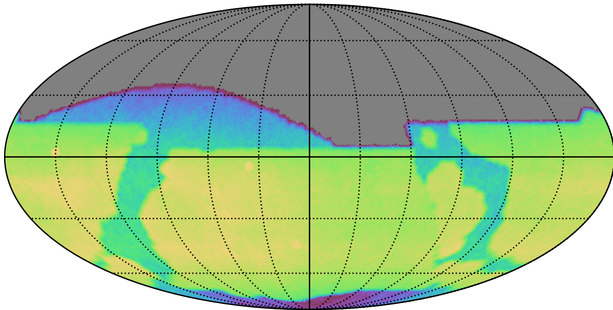
roll_pause_mjdp0_v3.4_10yrs All sky r band: CoaddM5
