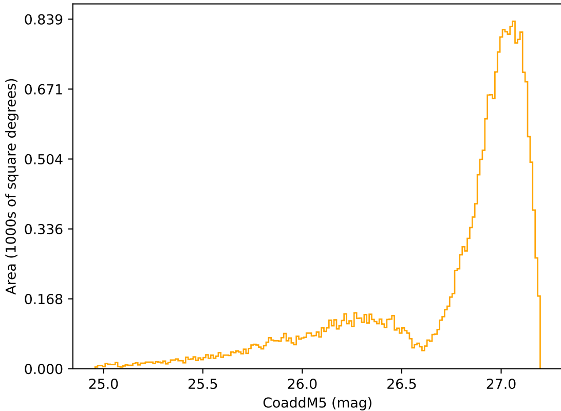
roll_pause_mjdp0_v3.4_10yrs All sky r band: CoaddM5
