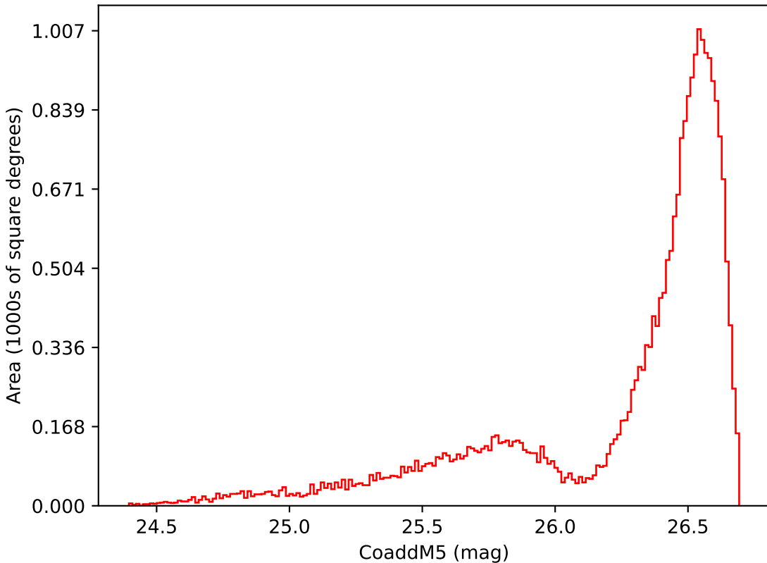
roll_pause_mjdp0_v3.4_10yrs All sky i band: CoaddM5
