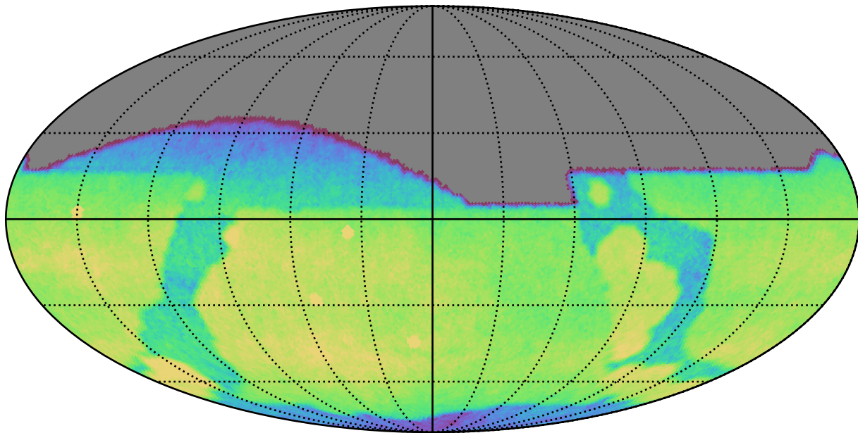
roll_pause_mjdp0_v3.4_10yrs All sky g band: CoaddM5
