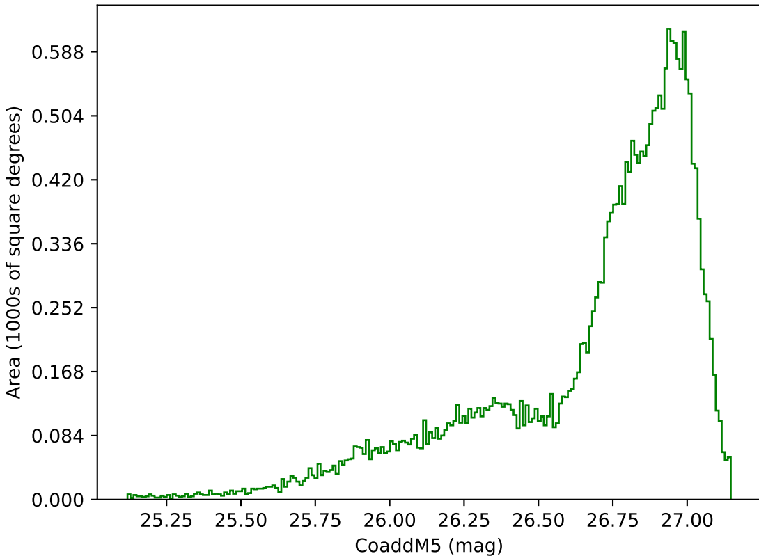
roll_pause_mjdp0_v3.4_10yrs All sky g band: CoaddM5
