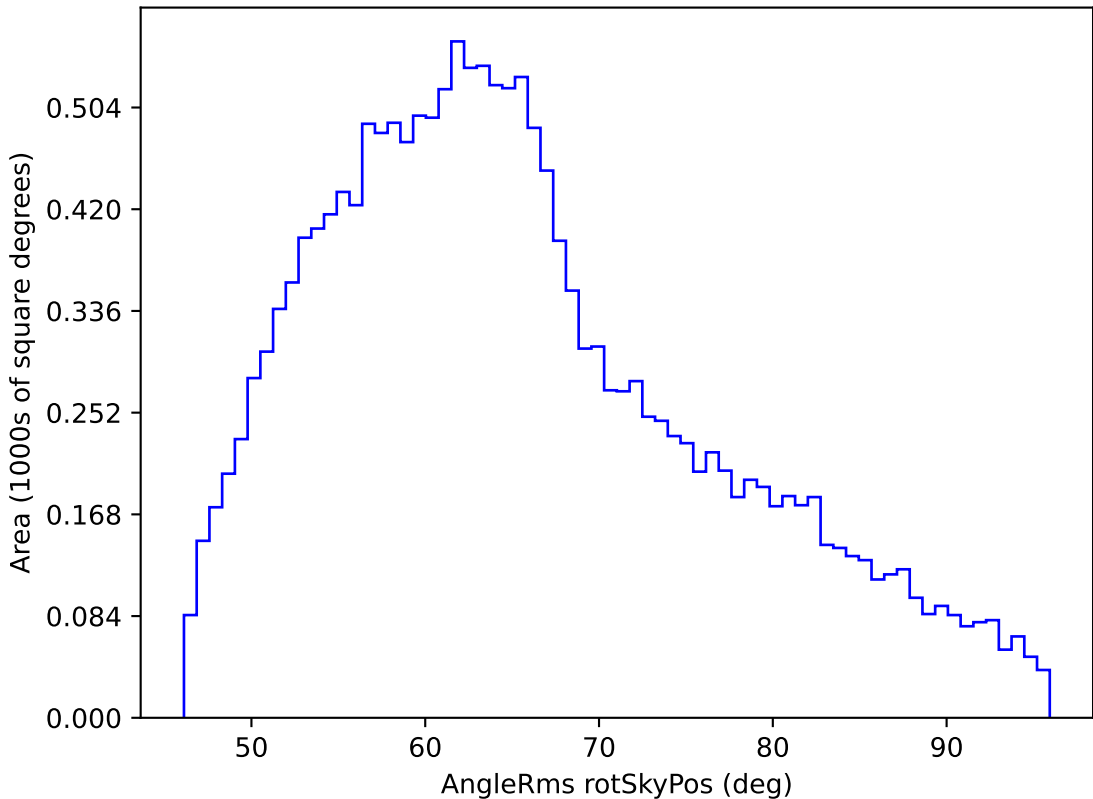
roll_pause_mjdp0_v3.4_10yrs WFD z band: AngleRms rotSkyPos
