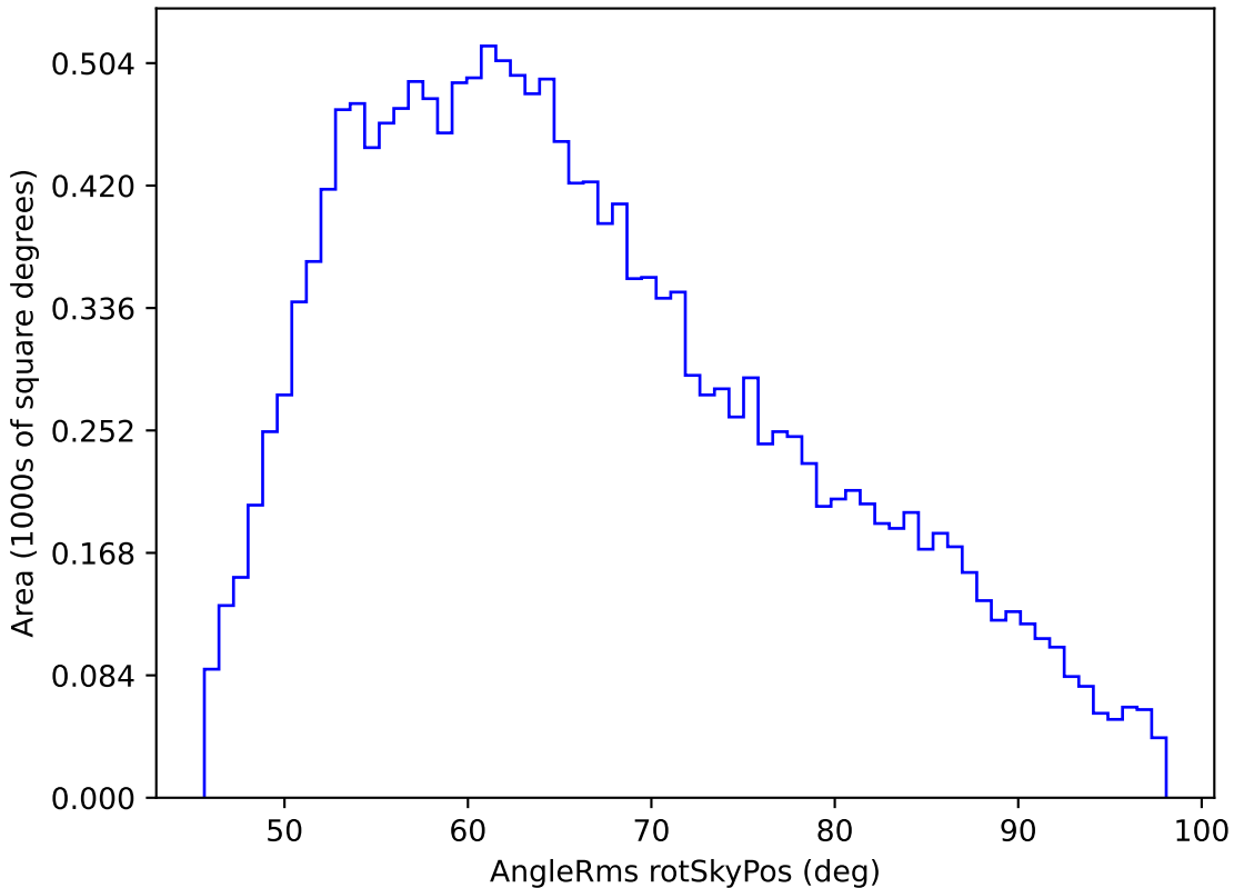
roll_pause_mjdp0_v3.4_10yrs WFD u band: AngleRms rotSkyPos
