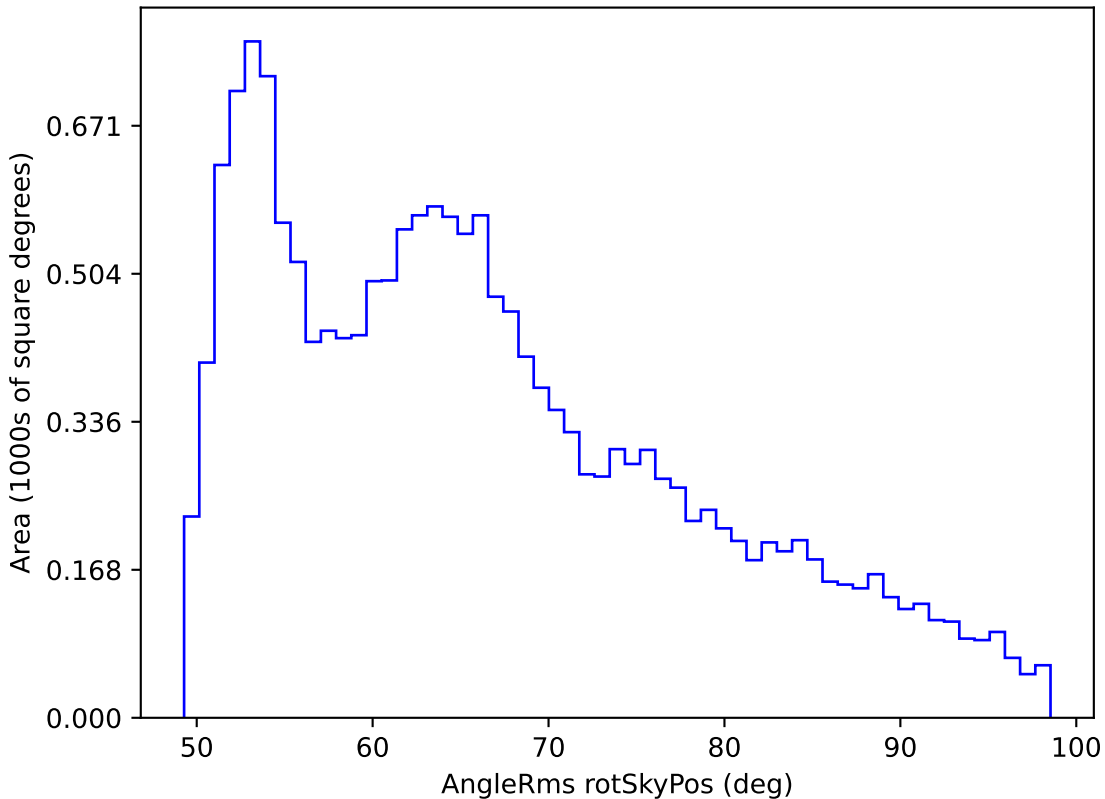
roll_pause_mjdp0_v3.4_10yrs WFD r band: AngleRms rotSkyPos
