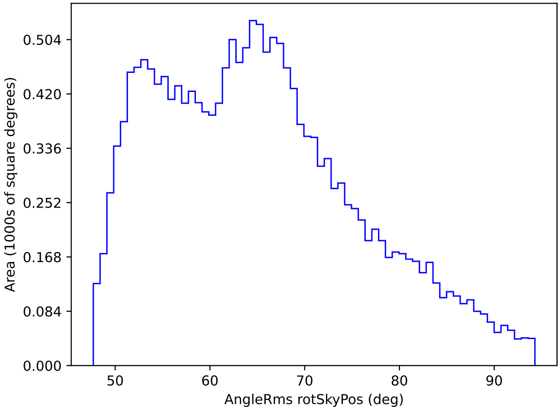
roll_pause_mjdp0_v3.4_10yrs WFD i band: AngleRms rotSkyPos
