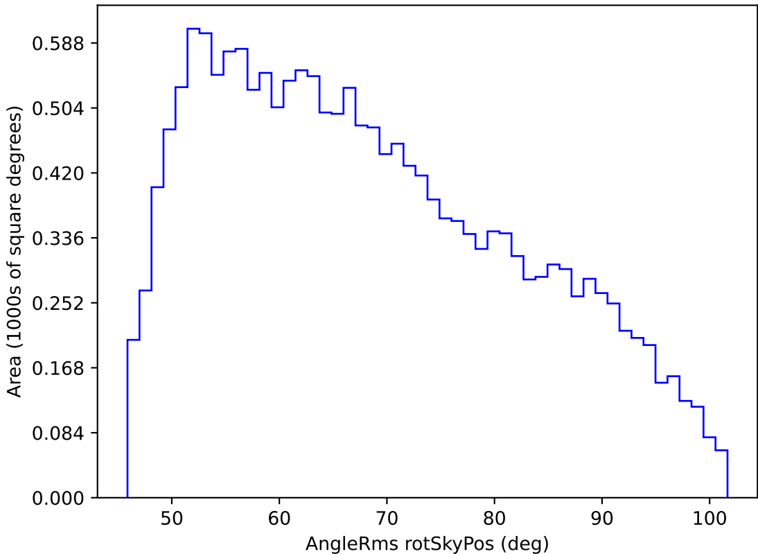
roll_pause_mjdp0_v3.4_10yrs WFD g band: AngleRms rotSkyPos
