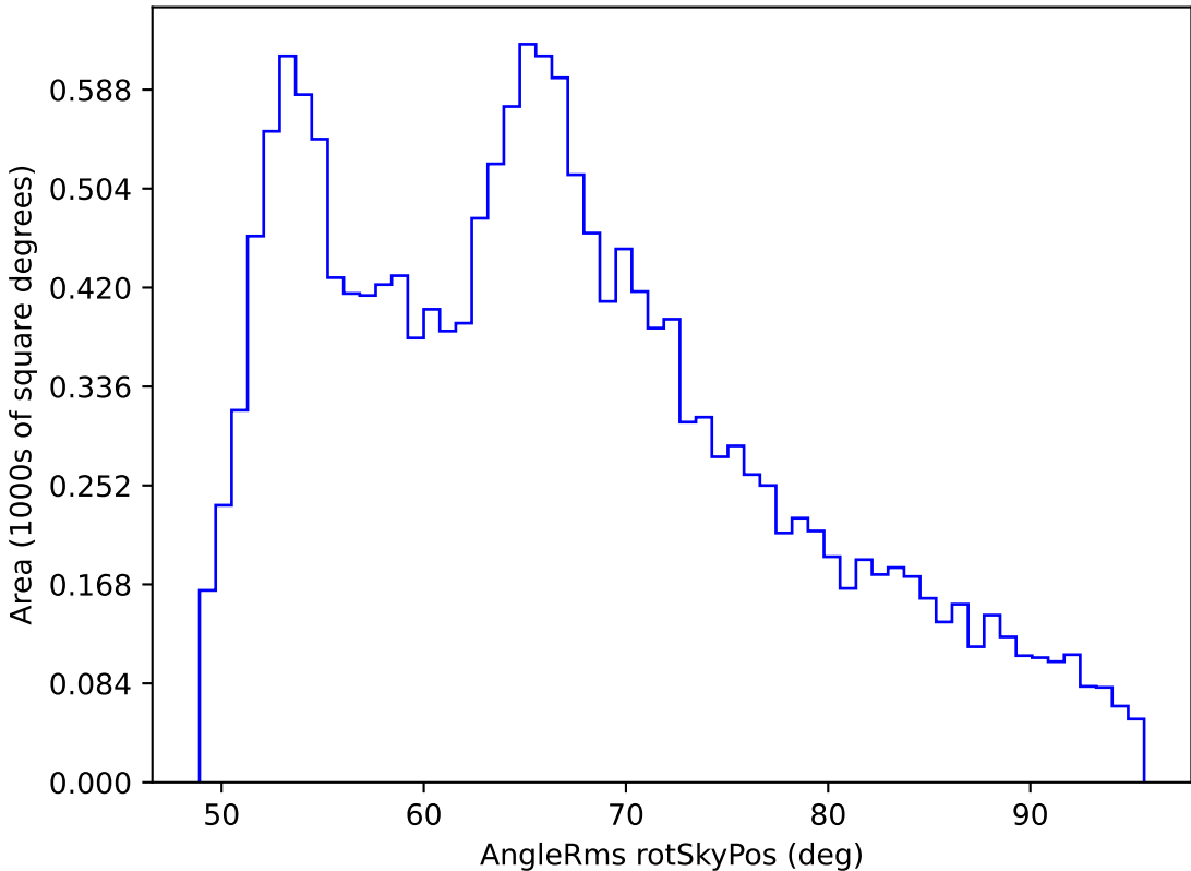
roll_pause_mjdp0_v3.4_10yrs WFD all bands: AngleRms rotSkyPos
