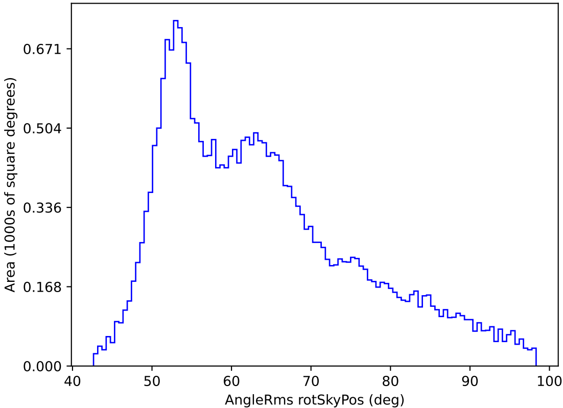
roll_pause_mjdp0_v3.4_10yrs All sky r band: AngleRms rotSkyPos
