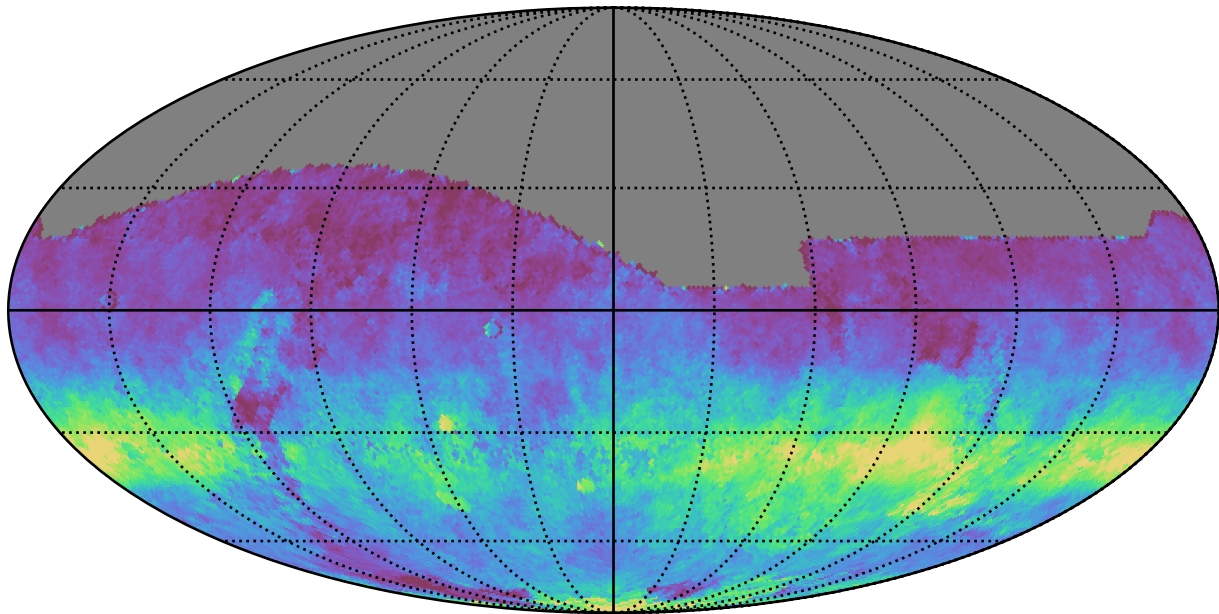
roll_pause_mjdp0_v3.4_10yrs All sky i band: AngleRms rotSkyPos
