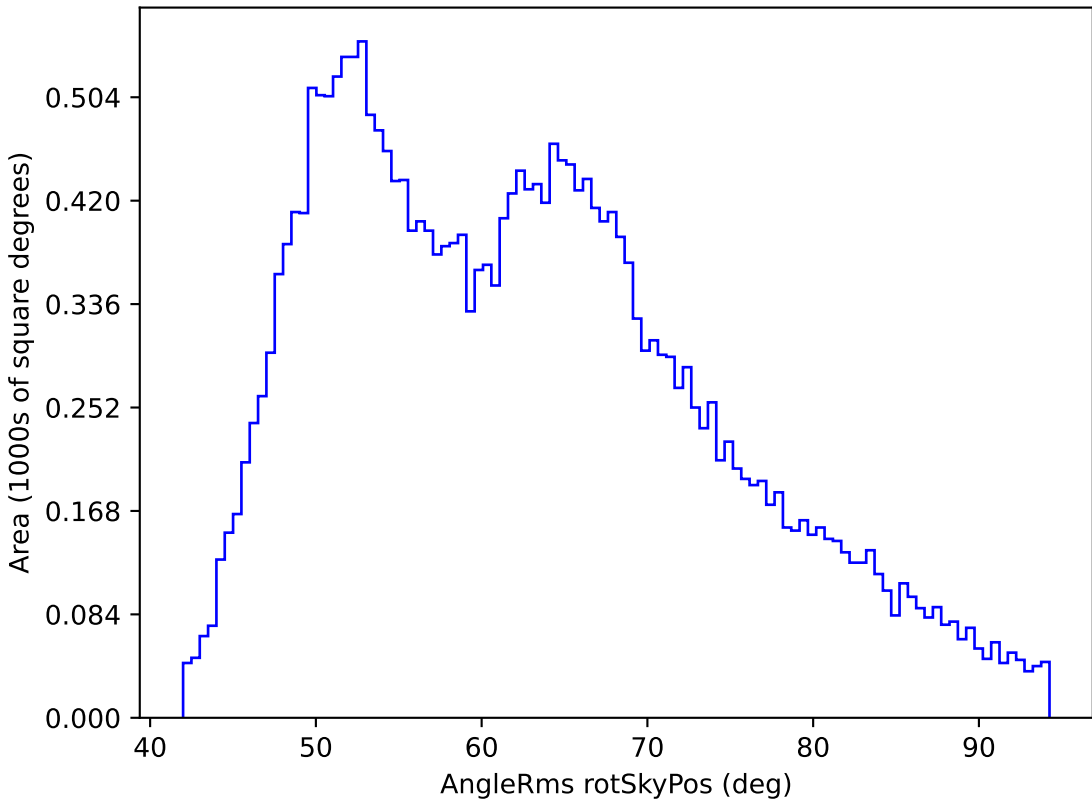
roll_pause_mjdp0_v3.4_10yrs All sky i band: AngleRms rotSkyPos
