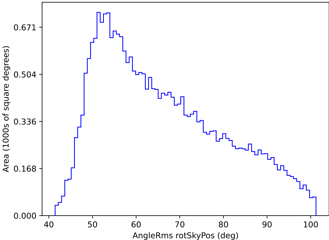
roll_pause_mjdp0_v3.4_10yrs All sky g band: AngleRms rotSkyPos
