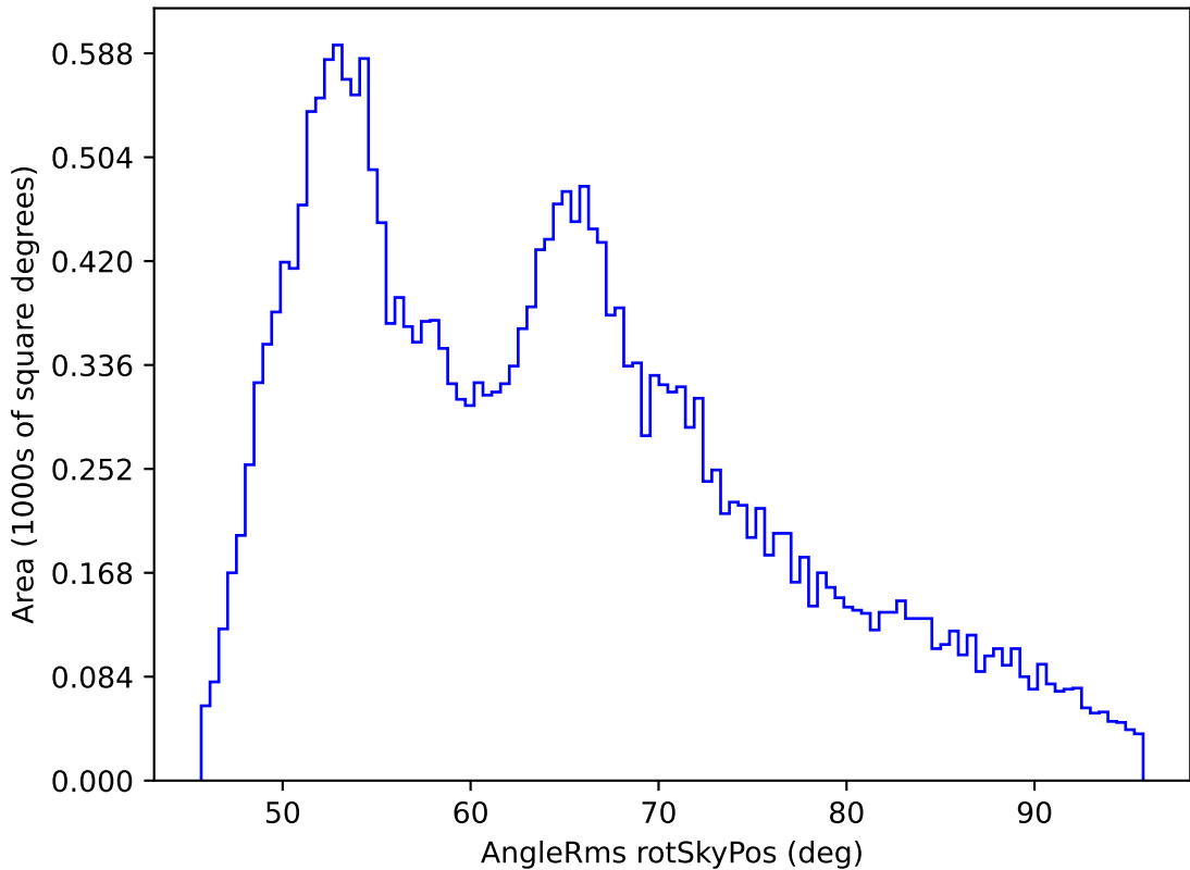
roll_pause_mjdp0_v3.4_10yrs All sky all bands: AngleRms rotSkyPos
