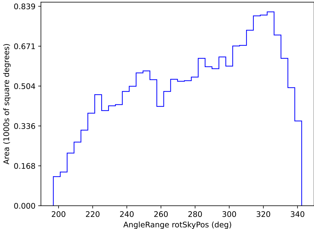
roll_pause_mjdp0_v3.4_10yrs WFD z band: AngleRange rotSkyPos
