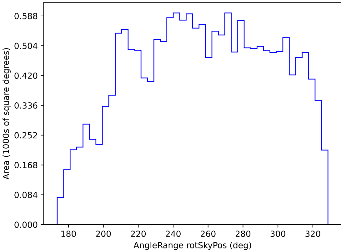
roll_pause_mjdp0_v3.4_10yrs WFD u band: AngleRange rotSkyPos
