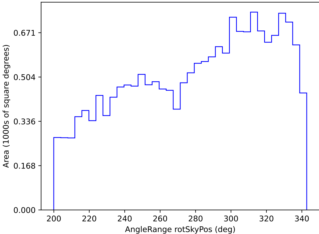
roll_pause_mjdp0_v3.4_10yrs WFD i band: AngleRange rotSkyPos
