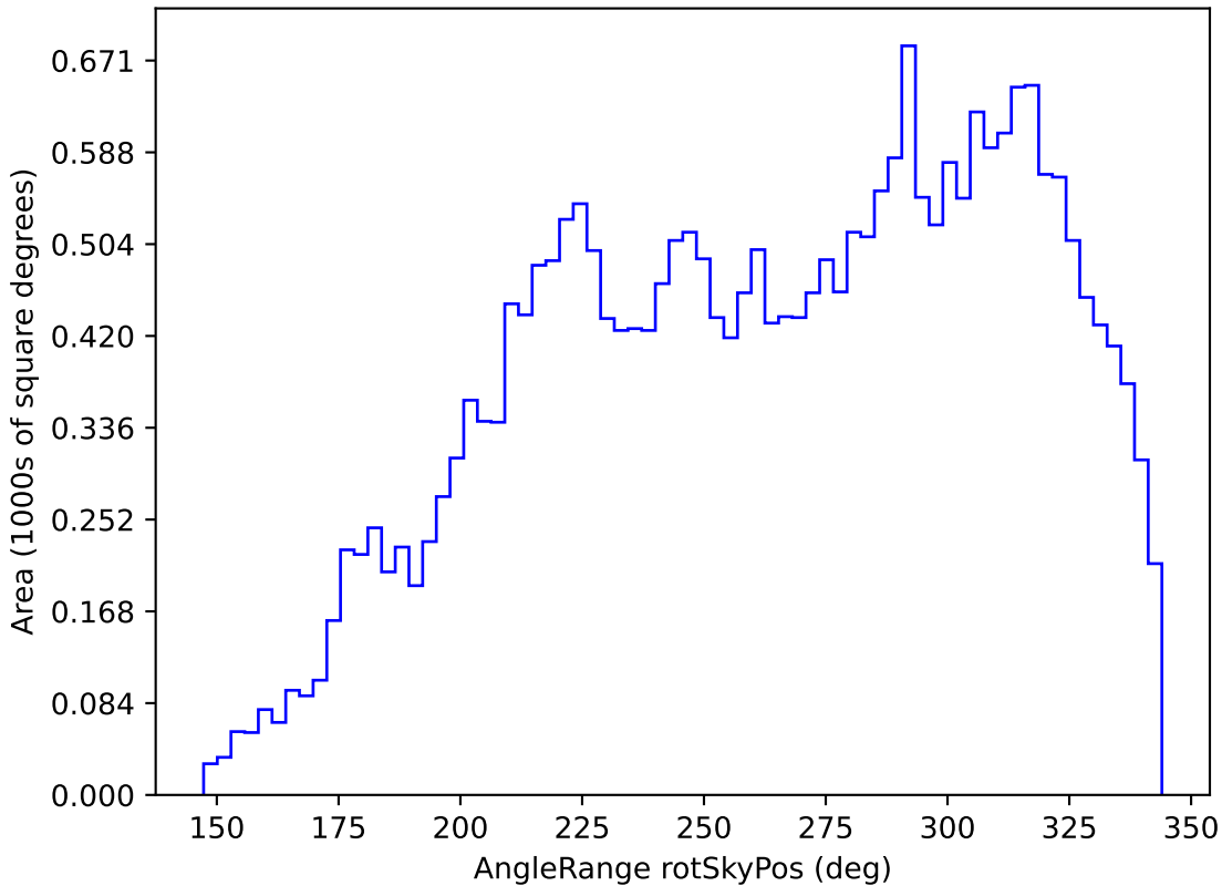
roll_pause_mjdp0_v3.4_10yrs All sky r band: AngleRange rotSkyPos
