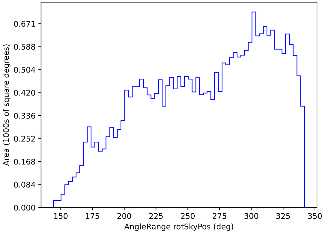
roll_pause_mjdp0_v3.4_10yrs All sky i band: AngleRange rotSkyPos
