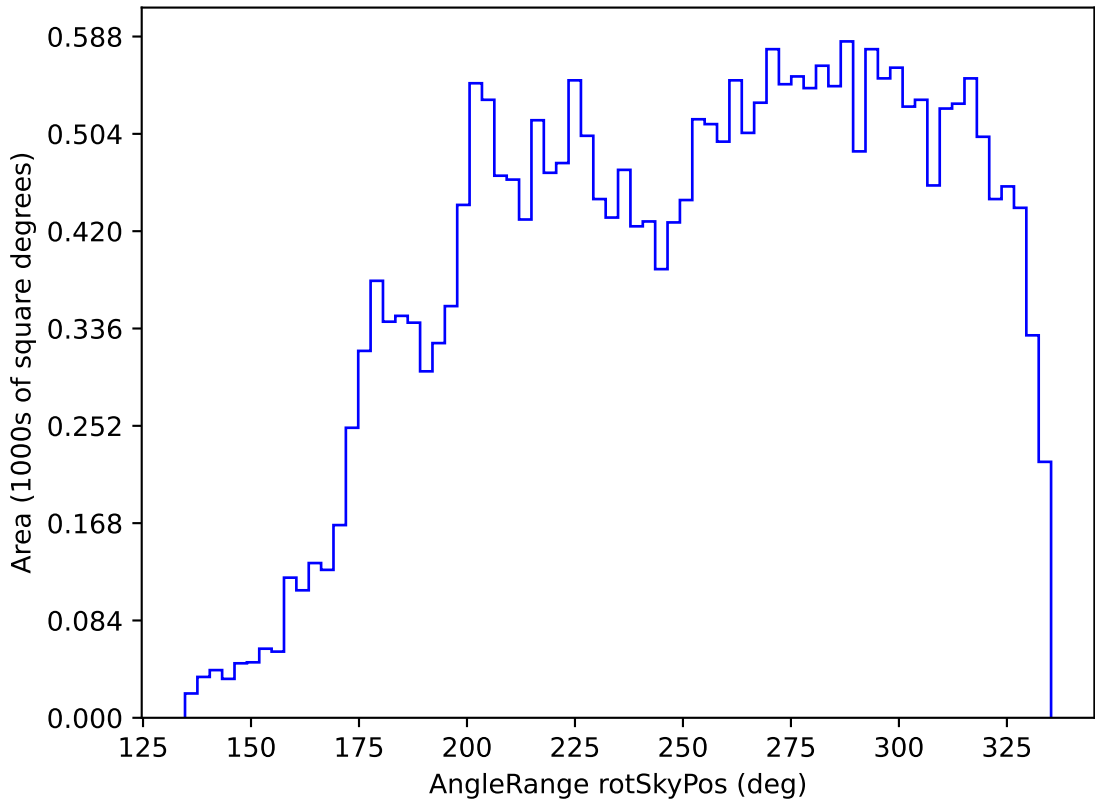
roll_pause_mjdp0_v3.4_10yrs All sky g band: AngleRange rotSkyPos
