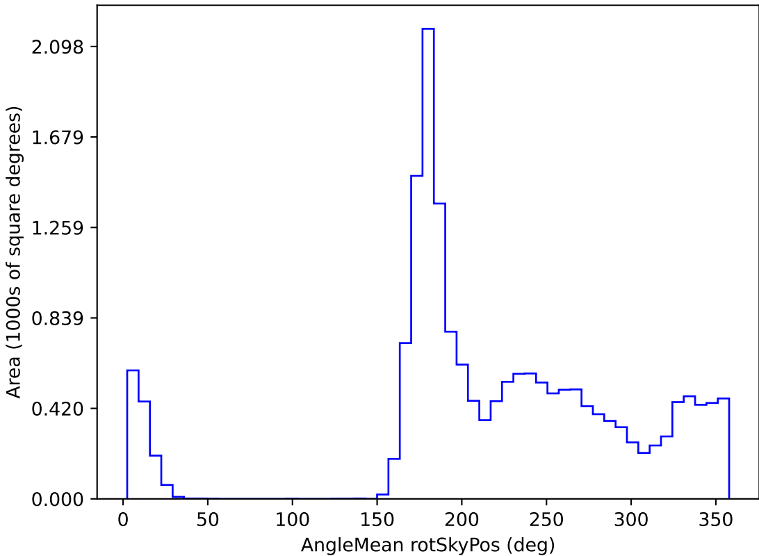
roll_pause_mjdp0_v3.4_10yrs WFD y band: AngleMean rotSkyPos
