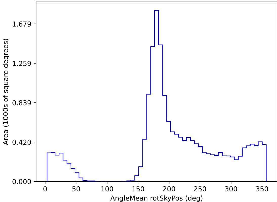
roll_pause_mjdp0_v3.4_10yrs WFD u band: AngleMean rotSkyPos
