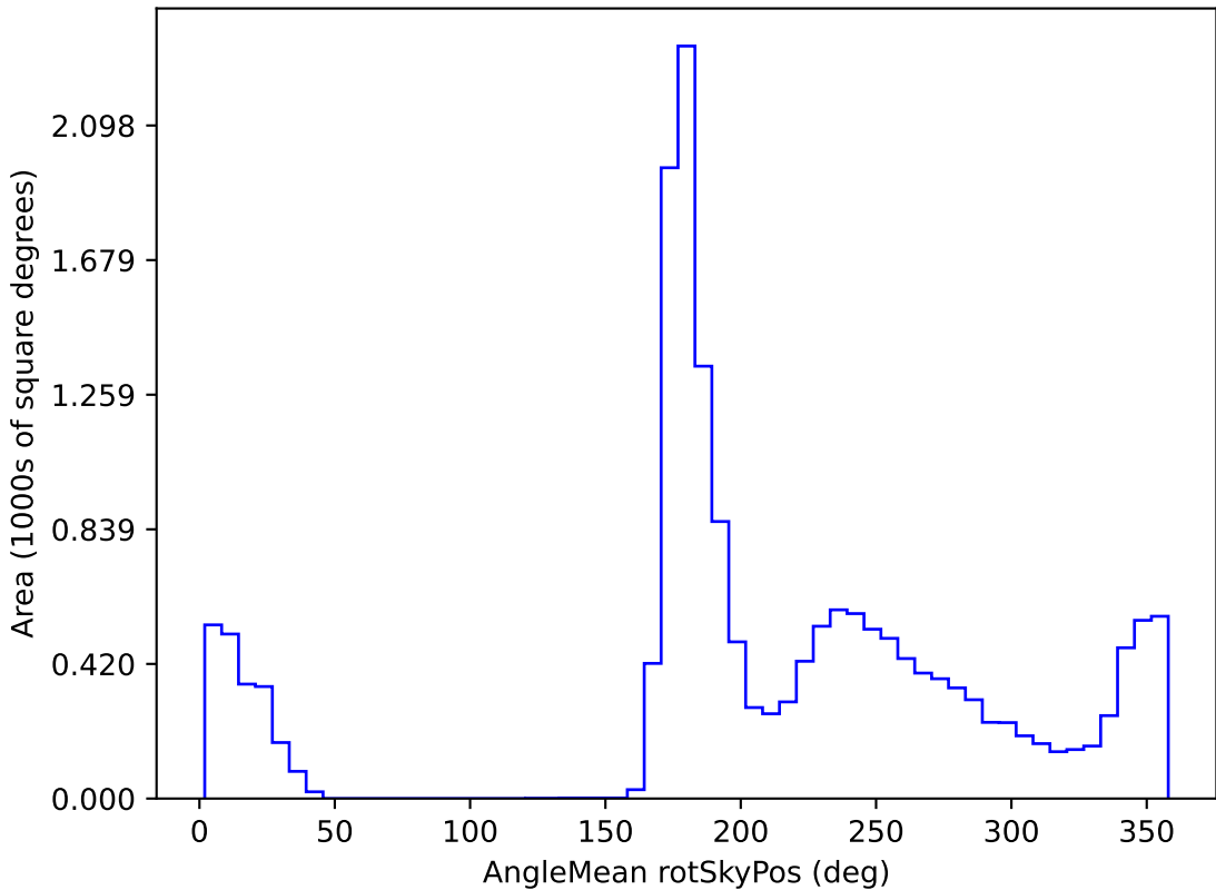
roll_pause_mjdp0_v3.4_10yrs WFD i band: AngleMean rotSkyPos
