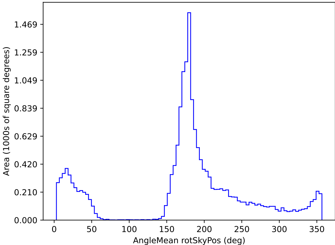
roll_pause_mjdp0_v3.4_10yrs WFD g band: AngleMean rotSkyPos
