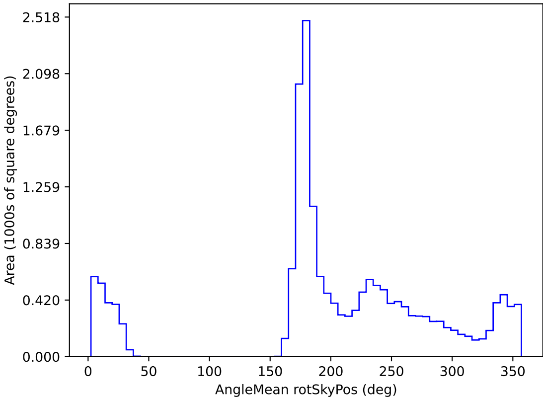
roll_pause_mjdp0_v3.4_10yrs WFD all bands: AngleMean rotSkyPos
