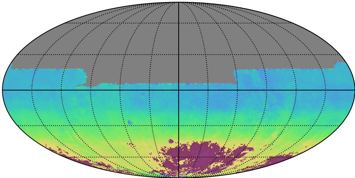
roll_pause_mjdp0_v3.4_10yrs All sky y band: AngleMean rotSkyPos
