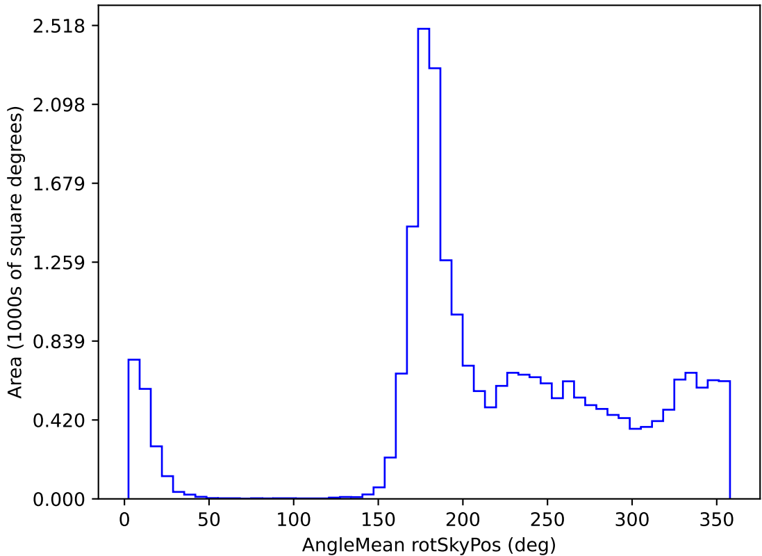
roll_pause_mjdp0_v3.4_10yrs All sky y band: AngleMean rotSkyPos
