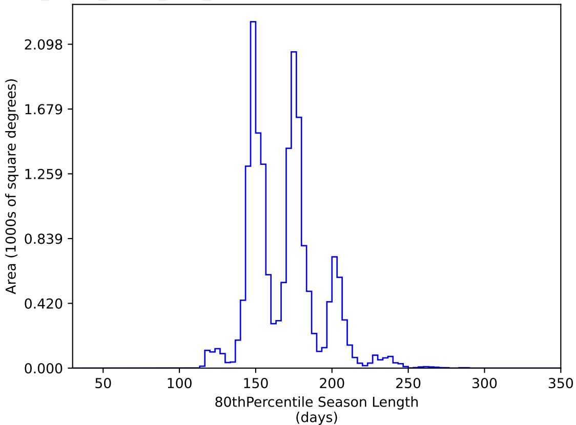
roll_pause_mjdp0_v3.4_10yrs WFD y band: 80thPercentile Season Length
