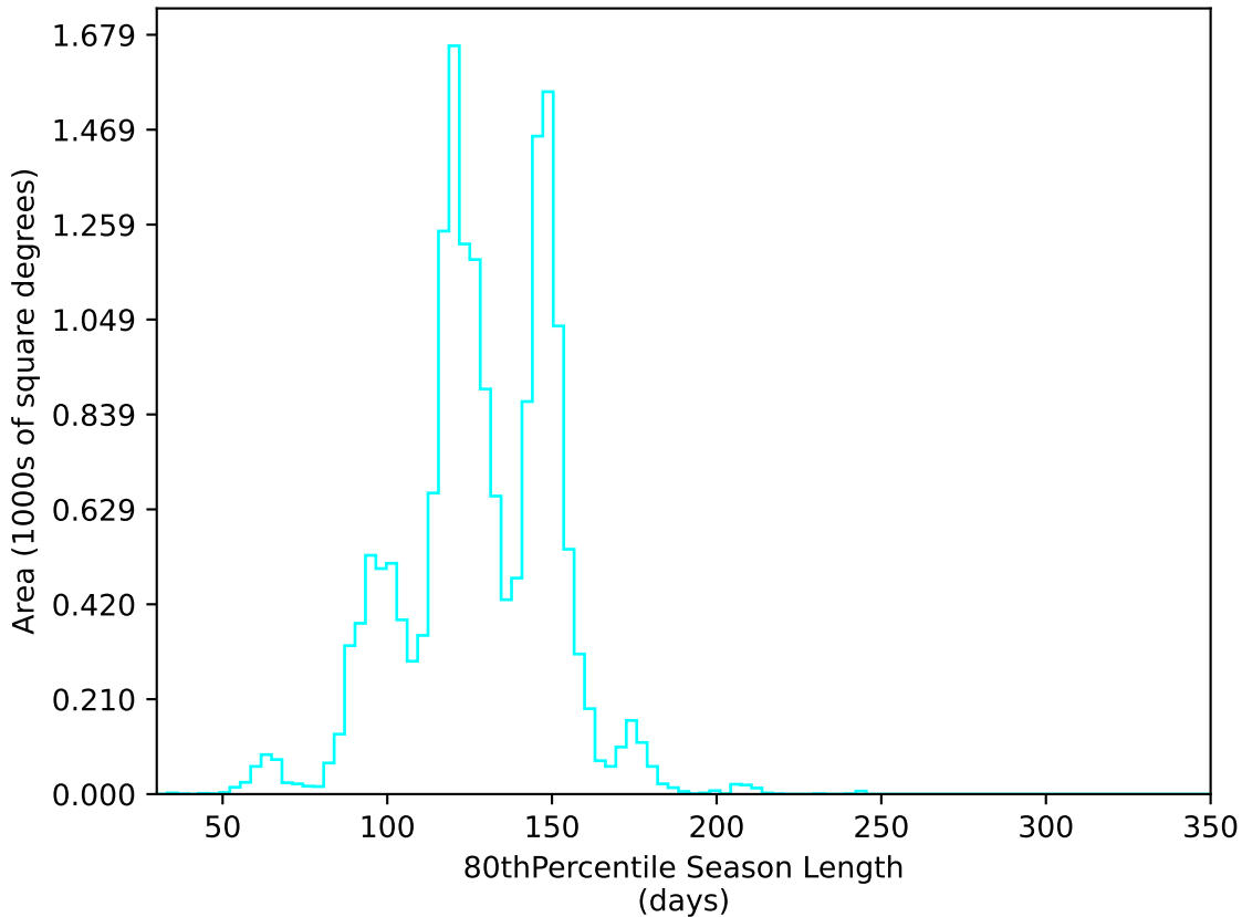
roll_pause_mjdp0_v3.4_10yrs WFD u band: 80thPercentile Season Length
