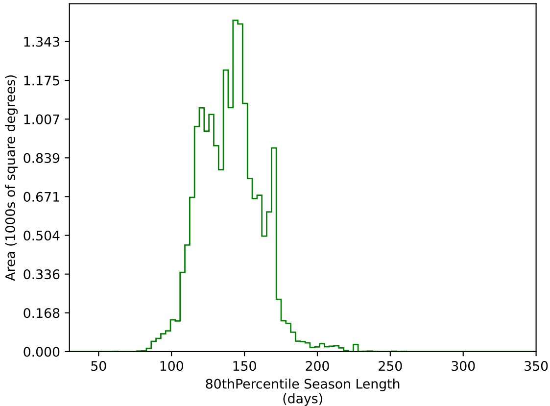
roll_pause_mjdp0_v3.4_10yrs WFD g band: 80thPercentile Season Length
