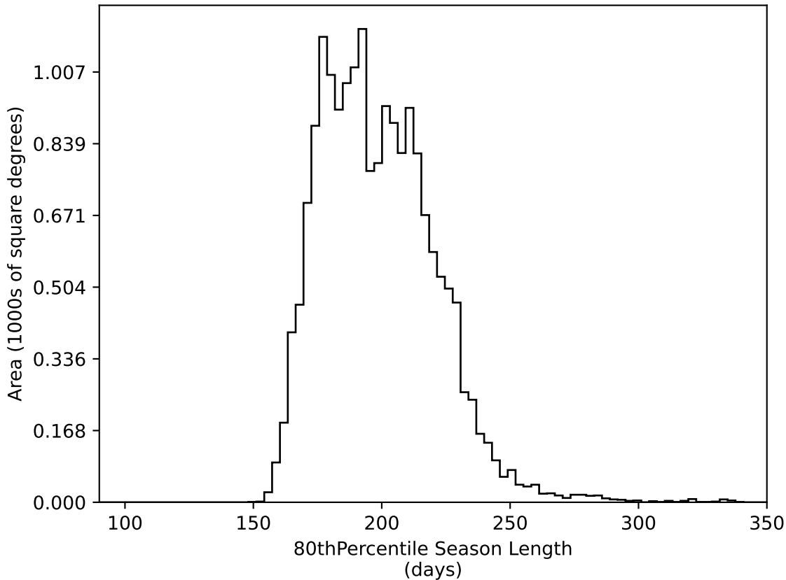
roll_pause_mjdp0_v3.4_10yrs WFD all bands: 80thPercentile Season Length
