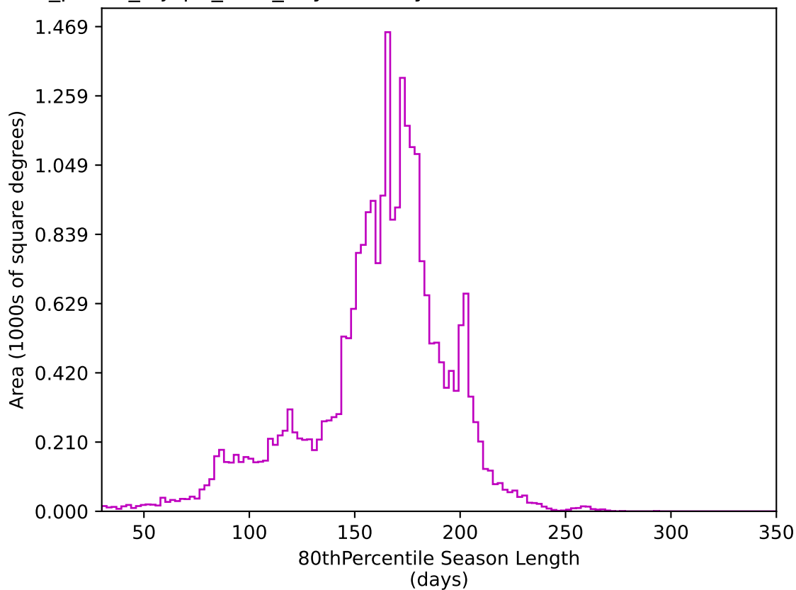
roll_pause_mjdp0_v3.4_10yrs All sky z band: 80thPercentile Season Length
