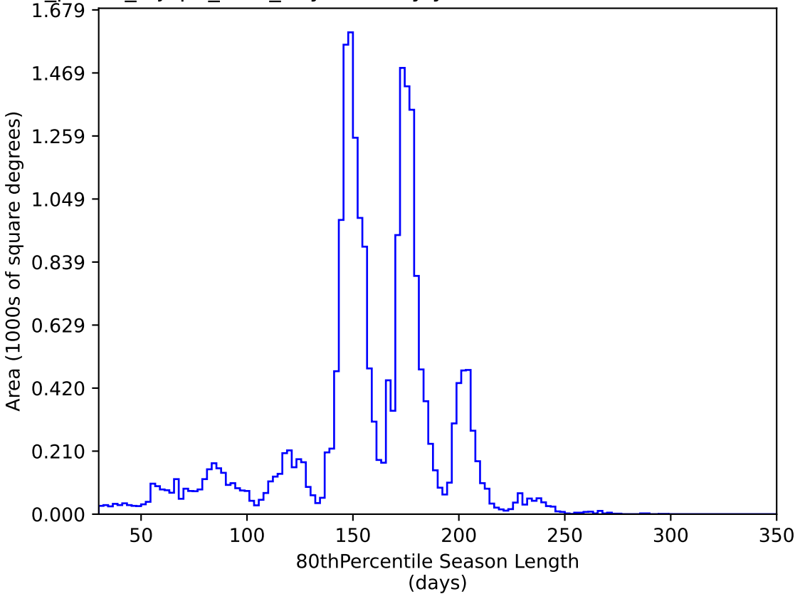
roll_pause_mjdp0_v3.4_10yrs All sky y band: 80thPercentile Season Length
