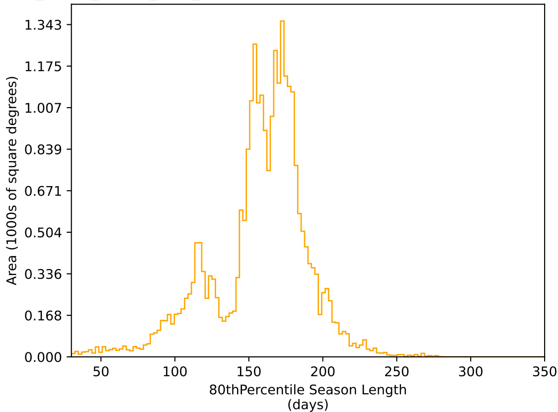
roll_pause_mjdp0_v3.4_10yrs All sky r band: 80thPercentile Season Length
