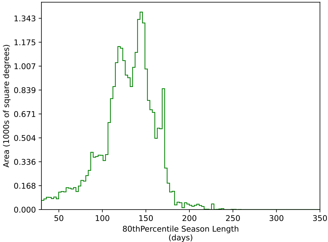
roll_pause_mjdp0_v3.4_10yrs All sky g band: 80thPercentile Season Length
