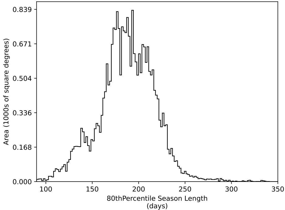
roll_pause_mjdp0_v3.4_10yrs All sky all bands: 80thPercentile Season Length
