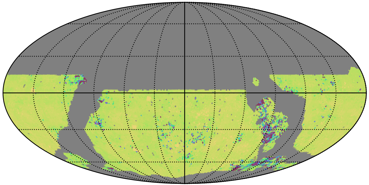
roll_pause_mjdp0_v3.4_10yrs WFD ug bands: 75th Percentile Intranight Timespan
