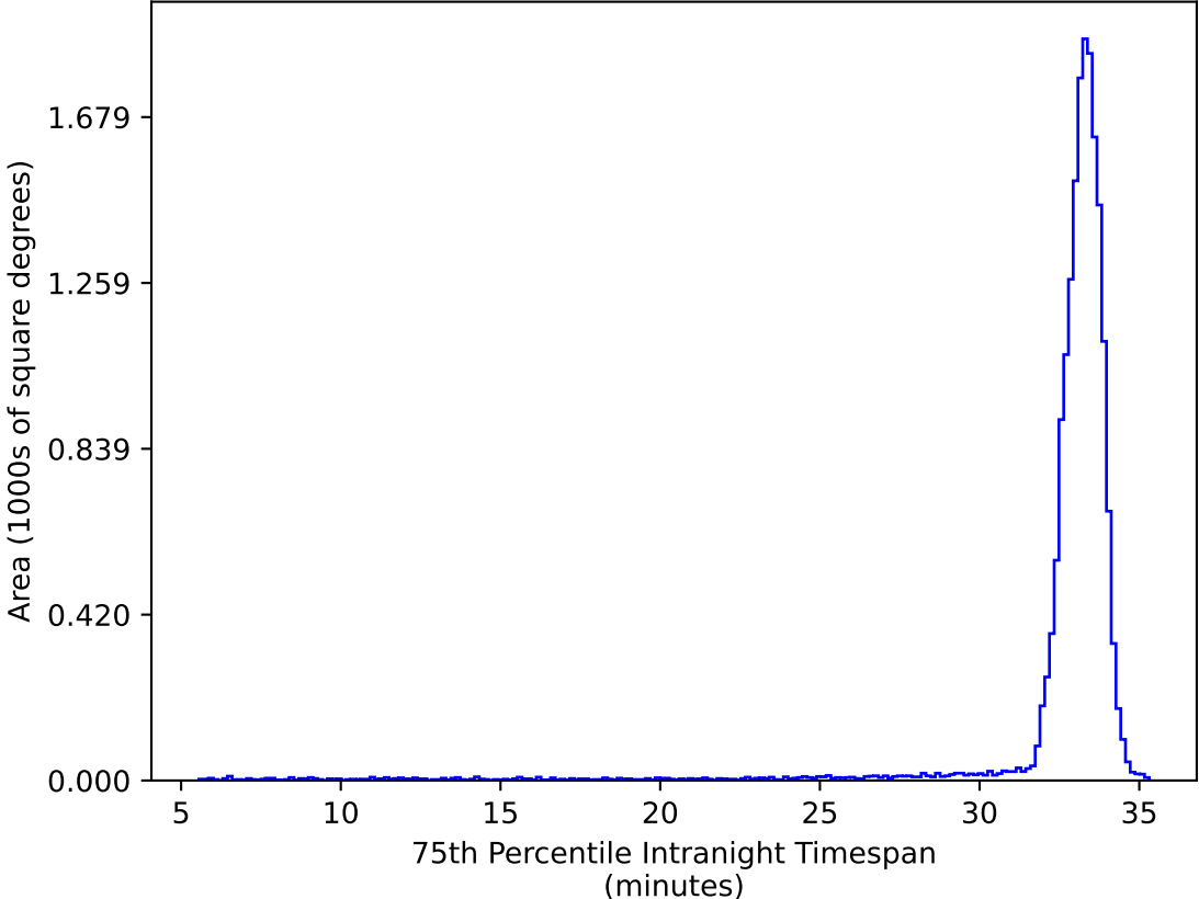
roll_pause_mjdp0_v3.4_10yrs WFD ug bands: 75th Percentile Intranight Timespan
