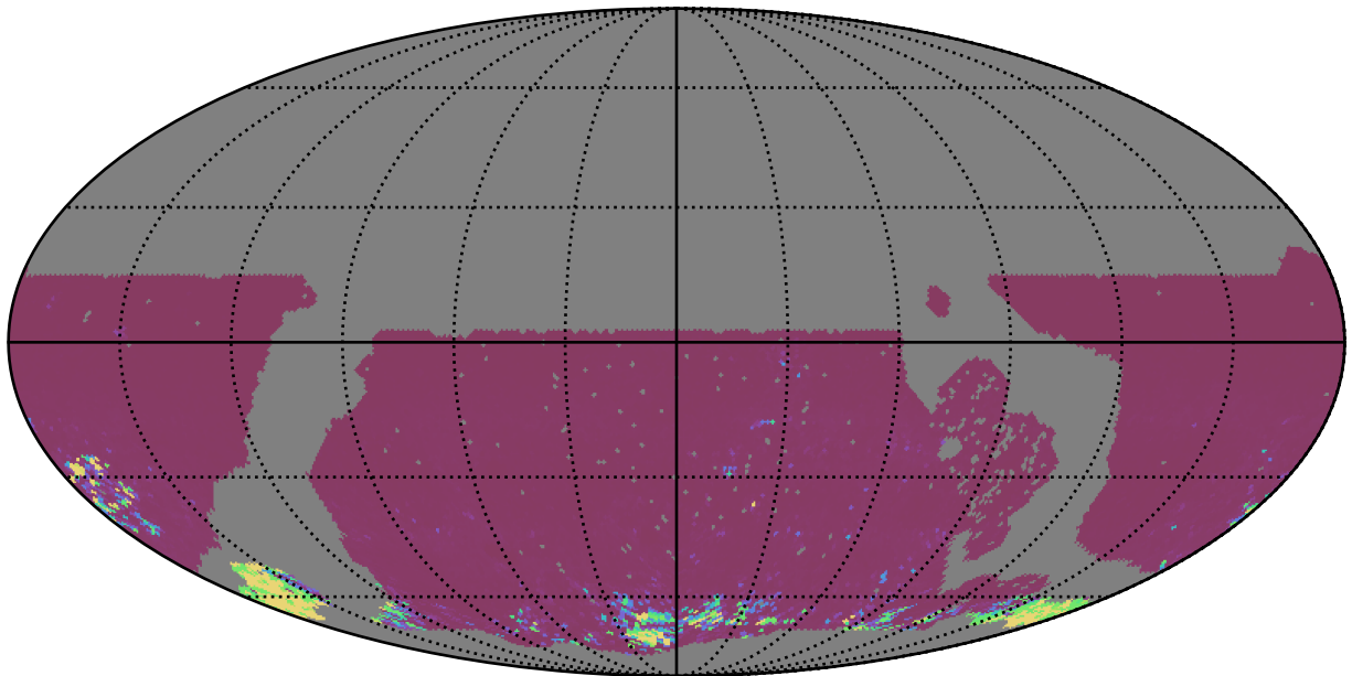
roll_pause_mjdp0_v3.4_10yrs WFD ri bands: 75th Percentile Intranight Timespan
